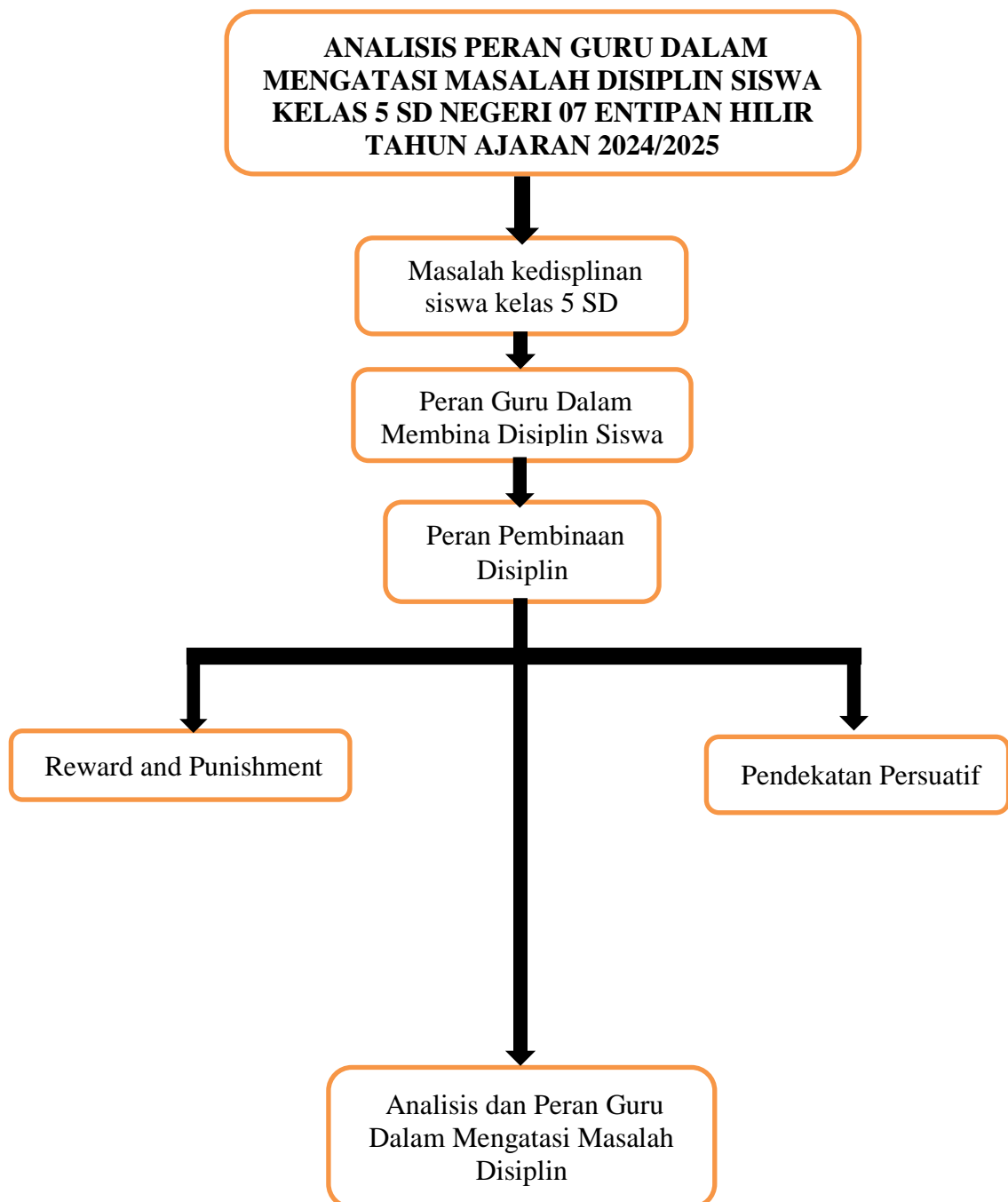
Gambar 2. 1 Alur Penelitian
